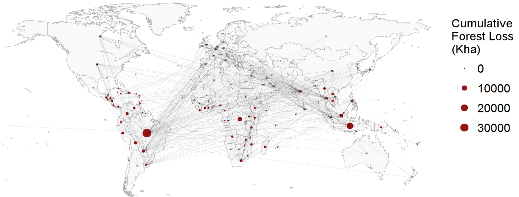
Fig. A6.2. The cumulative sum of annual forest loss detected 2000-2012 for pantropical countries (Hansen et al. 2013). Soybean export and import pathways associated with pantropical countries for the period 2000-2012 are shown without value weights for display purposes.
