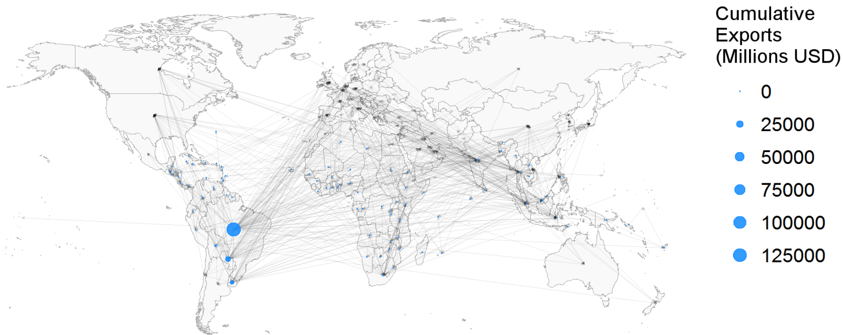
Fig. A6.3. The cumulative sum of soybean exports 2000-2012 from pantropical countries (Department of Economic and Social Affairs Statistics Division 2010, Food and Agriculture Organization of the United Nations 2016). Soybean export and import pathways associated with pantropical countries for the period 2000-2012 are shown without value weights for display purposes.
