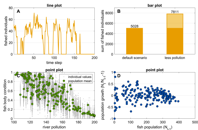
Fig. 4. Visualization of DemoViz (Box 1) results for one run over 200 time steps by X-Y plots. (A) Line plot showing the number of fished individuals vs. time (often referred to as time series). This number drops to zero during several periods. The (invisible) cause is that fishing is adaptive and stops when the population size falls below a threshold (cf. Box 1). (B) Bar plot comparing the total amount of fished individuals over the whole simulation period for two different scenarios. The visualization suggests that the intervention (reduced river pollution) is the cause for the higher amount of fishing, which is correct. (C) Point plots of the body condition of fish both at the individual and the population level (cf. legend) vs. river pollution. The visualization suggests a causal relationship from river pollution to body condition. This relationship exists, but is not that simple as pollution is not the only factor affecting body condition (cf. Fig. 2A). (D) Point plot of population growth vs. population size of the previous time step. It makes the causal relationship visible that large population sizes do not allow for high reproduction. However, for small population sizes reproduction can also be low, driven by different causes that are not shown.
