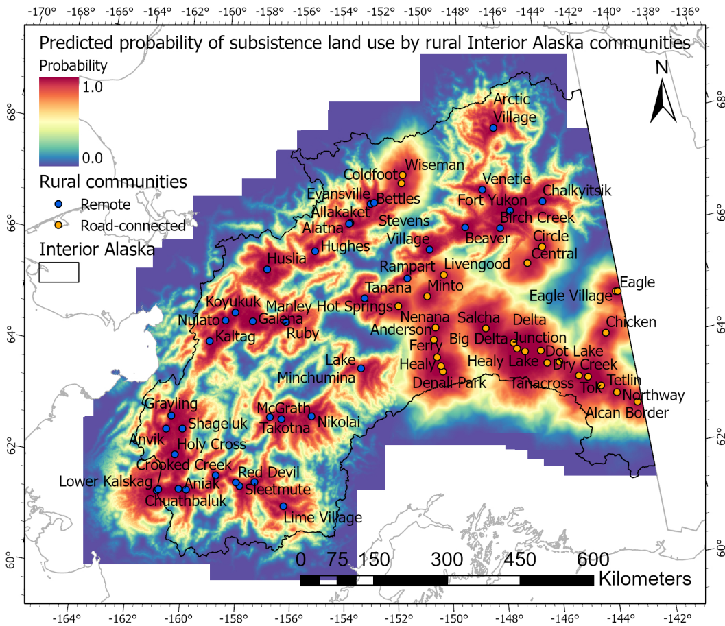
Fig. 7. Predicted probability of subsistence land use by rural Interior Alaska communities derived from logistic regression models. The regional composite was constructed from community-level model output using the maximum probability value (0 – 1.0) per pixel. These models likely underestimate the probability of subsistence land use, since they were derived from maps representing a single year of subsistence activity.
