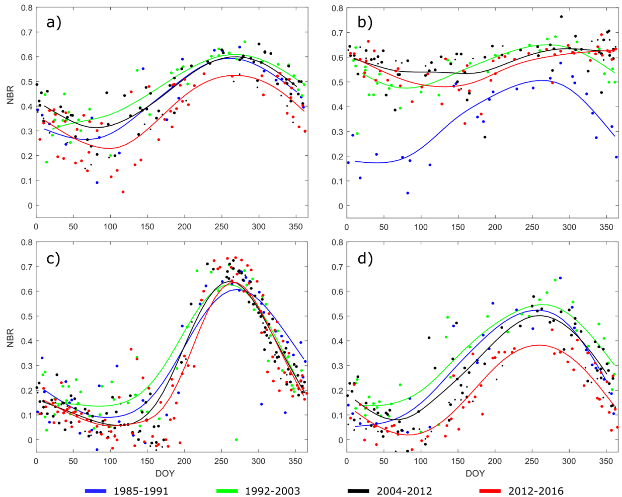
Fig. A1.4. Spline interpolation results for four pixels in our study area showing changes across political and management periods in a) shrublands, b) plantation forest, c) grazing land, and d) protected grassland. For example, the blue line (Derg period) demonstrates the seasonal pattern of the vegetation prior to the establishment of a plantation forest, while the green, black, and red lines are showing the seasonal pattern of the plantation forest in subsequent periods, which is far less variable. There are 70 images in the Derg period (44 with <50% cloud cover), 148 images in the Transition period (87 with <50% cloud cover), 147 images in the NGO period (86 with <50% cloud cover), and 232 in the Co-management period (135 with <50% cloud cover).
