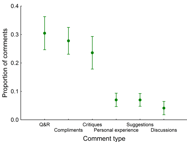
Fig. 7. Comparison of the means of proportions of comments in favor of hunting activity. Q&R = Questions for or requests to the uploader.
