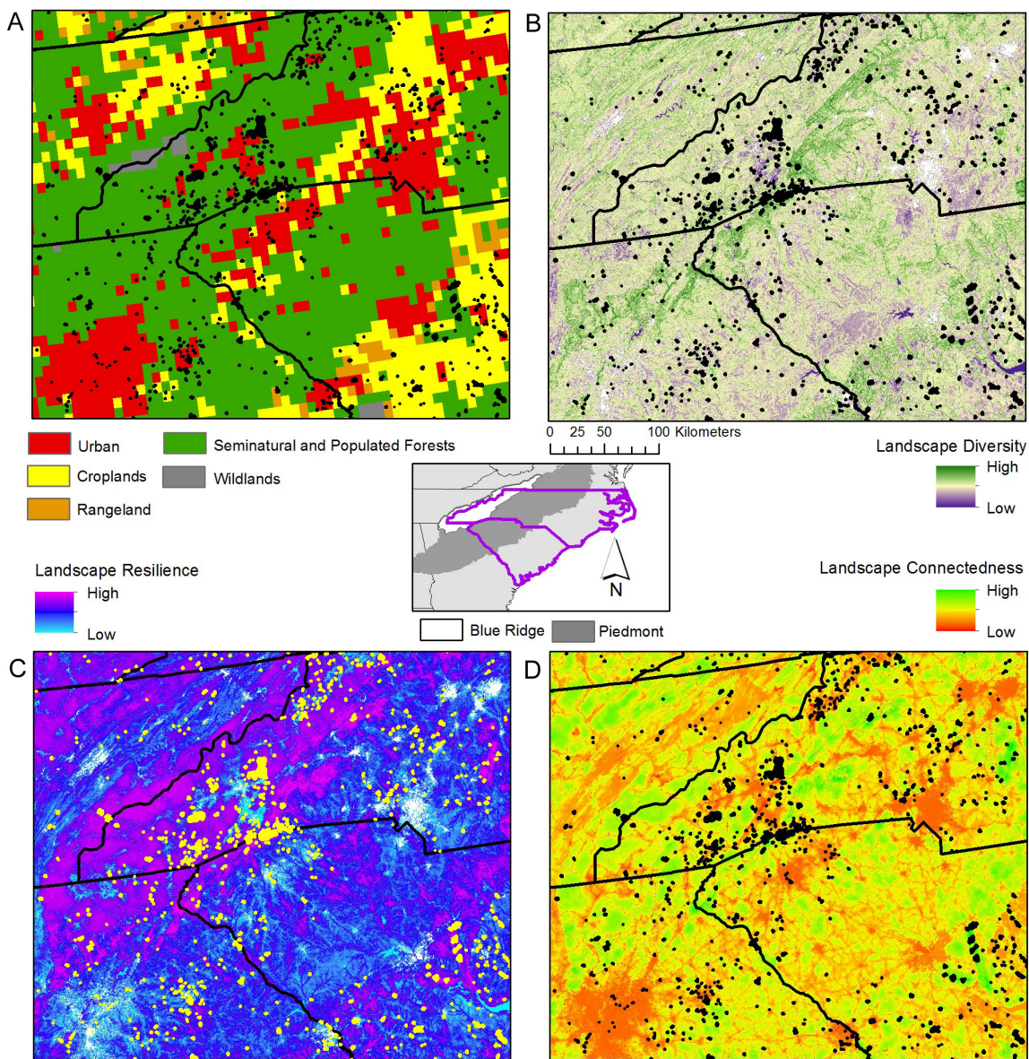
Fig. 3. Distribution of conservation easements (black outline) in the Southern Piedmont and Blue Ridge regions of North and South Carolina across (A) anthrome types (Ellis et al. 2010), (B) landscape diversity, (C) landscape resilience, and (D) landscape connectedness (Anderson et al. 2014).
